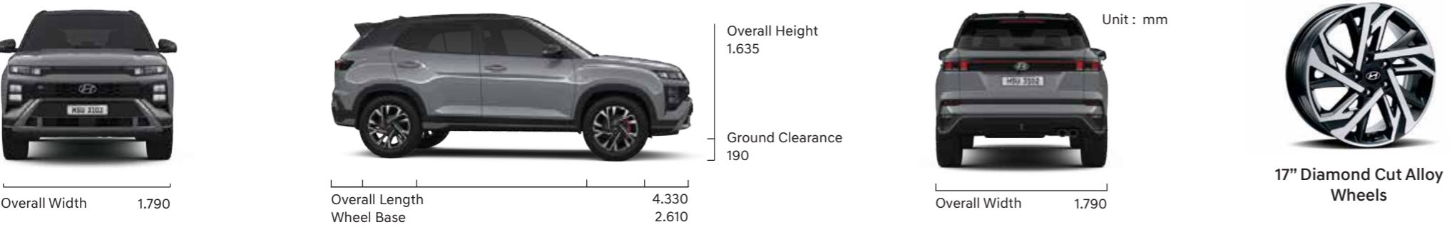
Overall Height 1.635 Ground Clearance 190 Overall Width 1.790 Overall Length 4.330 Wheel Base 2.610 Unit : mm 17" Diamond Cut Alloy Wheels
